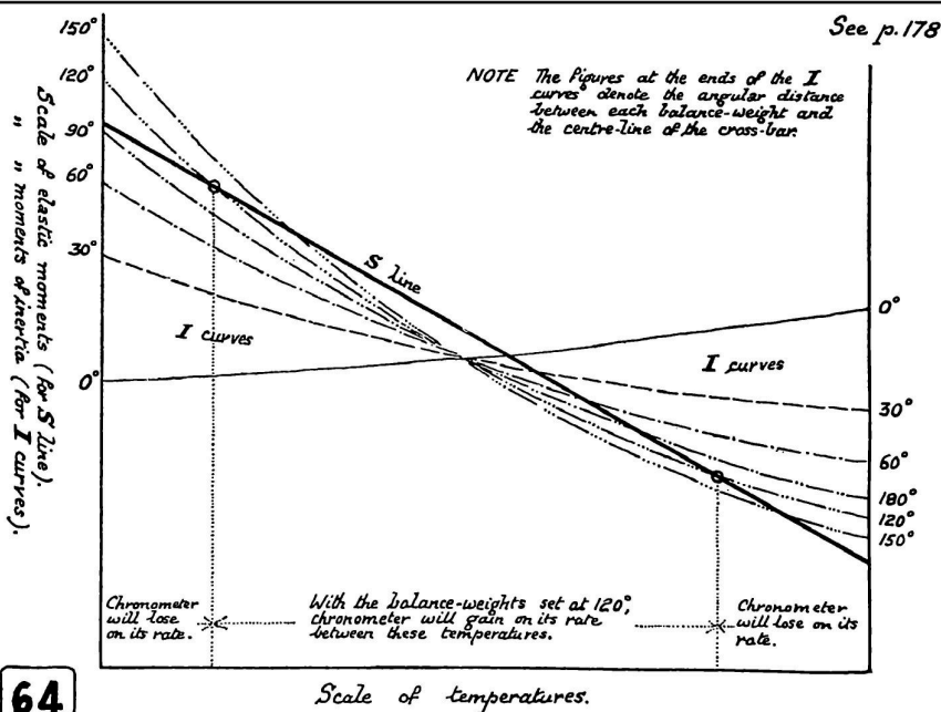
Diagram showing effect of compensation, and cause of "middle temperature error"
