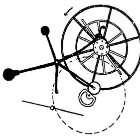
IV. \frac{1}{4} second later. Re-winding completed. Detent has returned to its original position, fifth wheel is again locked by the short arm, the next pin is about to enter the claw.
