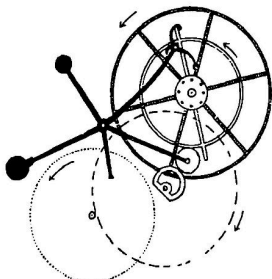
III. \frac{1}{4} second later. Fifth wheel has been unlocked, and has completed half its revolution. Cam has moved detent further anti-clockwise, and released claw from pin. Fly is spinning.
