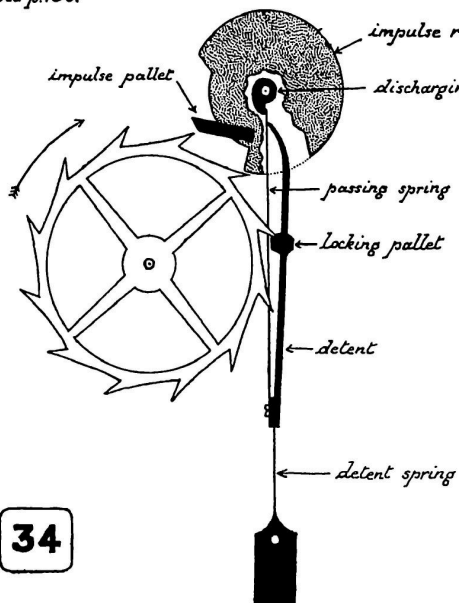
Earnshaw's spring-detent escapement. [1784]
