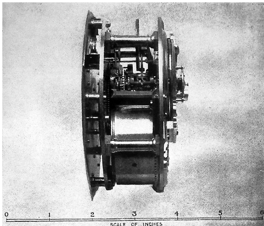
Plate 18 SIDE-VIEW OF MUDGE'S FIRST TIMEKEEPER
