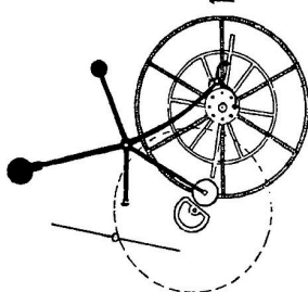
I. The contrate wheel is in motion, and the remainder of the mechanism locked the stop on the fifth wheel being in contact with the short arm of the detent. A pin is just entering the claw.
