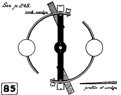
How to wedge a balance.
