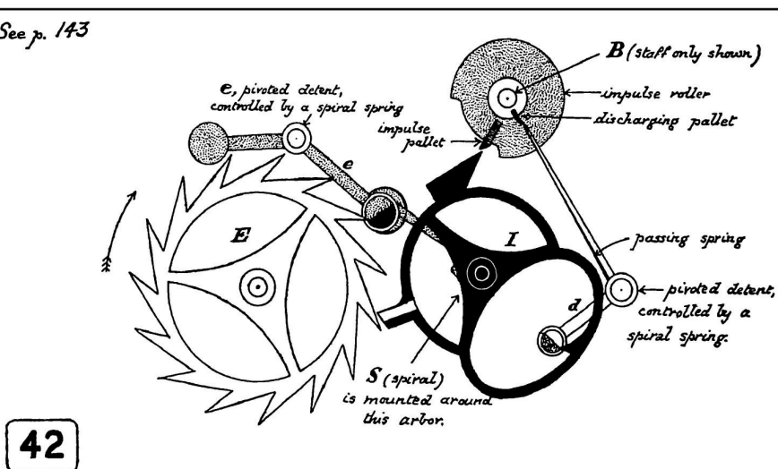
Pettavel's constant-force escapement.
