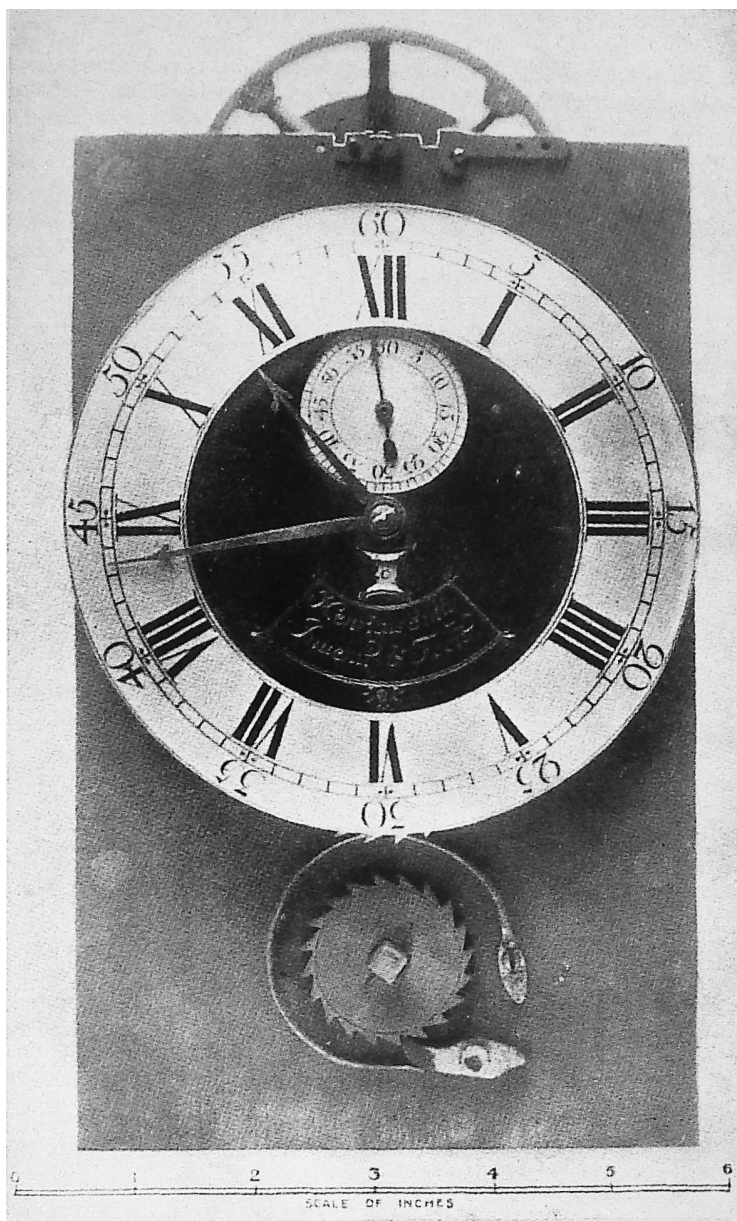
Plate 2 MOVEMENT OF ONE OF SULLY'S MARINE CLOCKS
