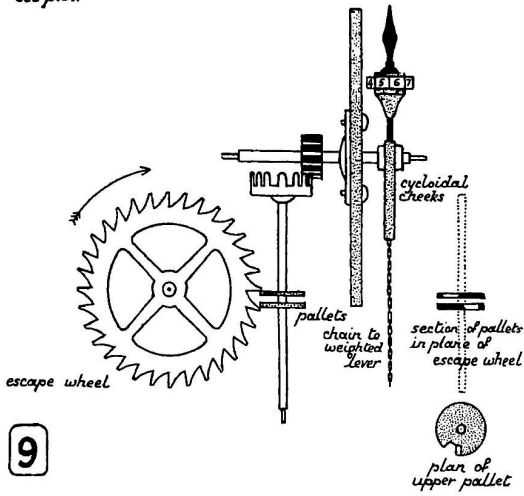
Escapement of Sully's marine clock. [See also Plate III.]
