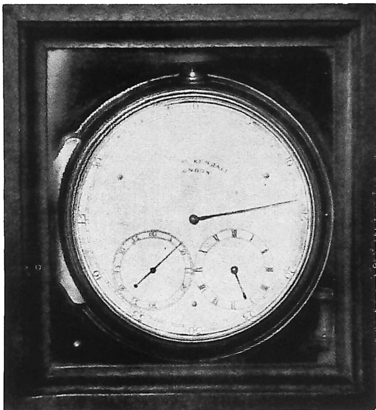
Plate 16 THE "BOUNTY'S" TIMEKEEPER (K2)
