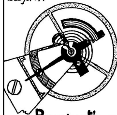
Breguet's com- -pensation curb.
