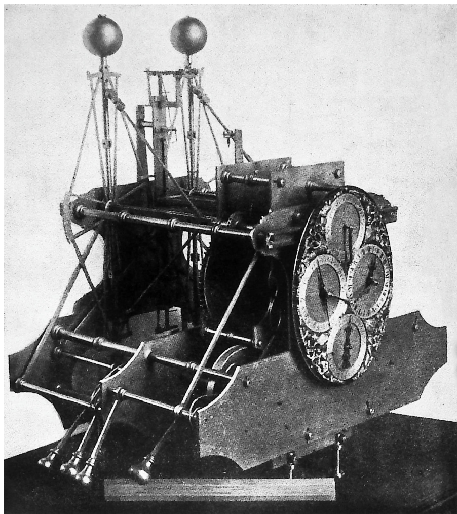
Plate 7 THREE-QUARTER VIEW OF HARRISON'S NO. 1
