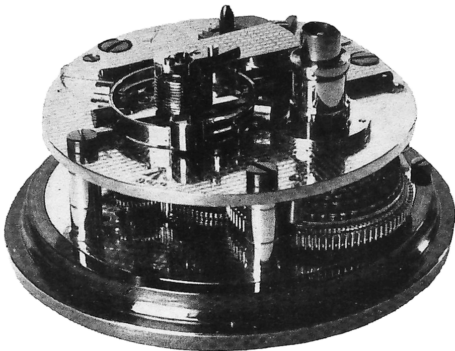
Plate 39 TYPICAL MODERN CHRONOMETER MOVEMENT
