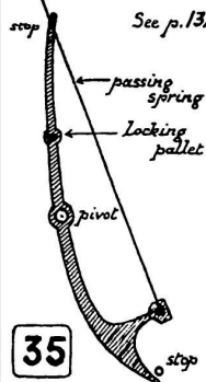
Motel's pivoted detent.
