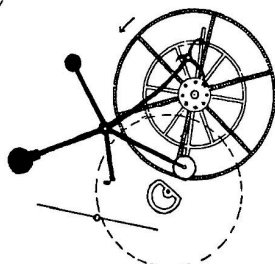
II. 7 seconds later. The detent has been turned slightly anti-clockwise by the pin, and the short arm is just about to clear the stop.
