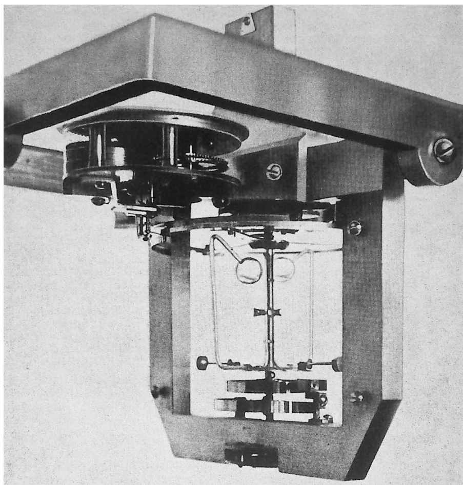
Plate 22 MOVEMENT OF LE ROY'S "MONTRE MARINE"
