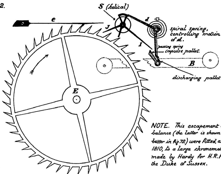
Hardy's constant-force escapement [1810].
