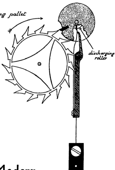
Modern chronometer escapement.
