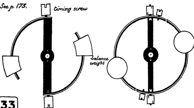
Earnshaw's compensation balance
