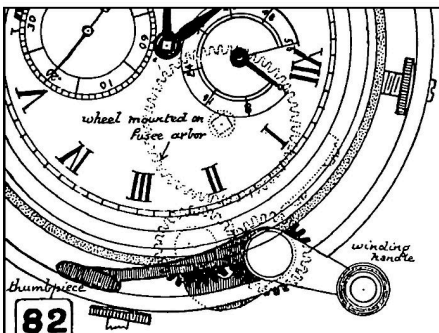
Britten's winding gear.
