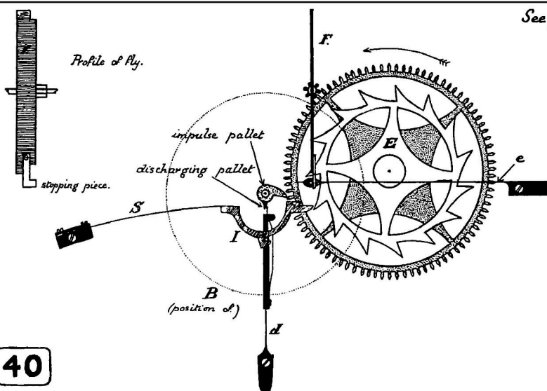
Breguet's constant-force escapement [1795].
