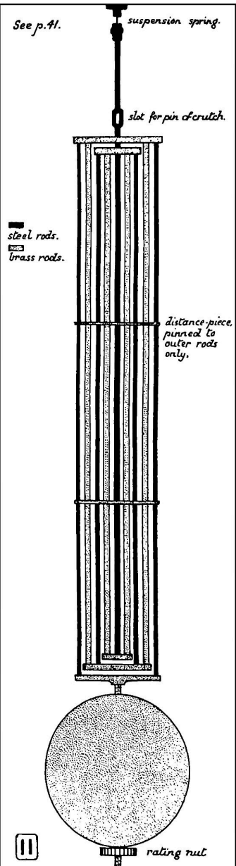
Harrison's "gridiron" pendulum.
