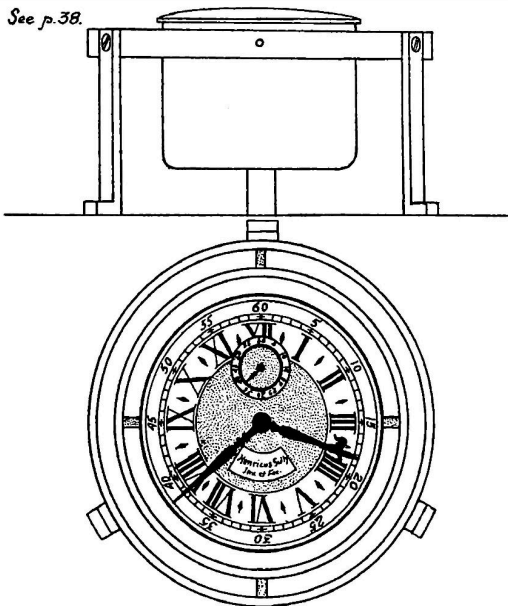
Sully's marine watch.
